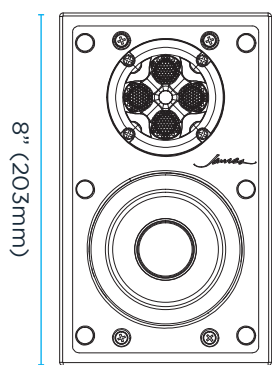
4.625" (117mm) Cut-Out Diameter Front View
