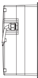
3.86" (98mm) Mounting Depth + Enclosure Side View
